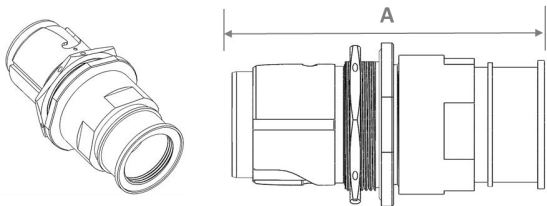
Jam nut shell with cable gland
