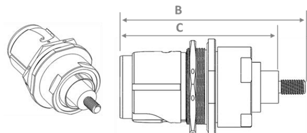
Wall mount Jam Nut receptacle with screw contact (external thread)
